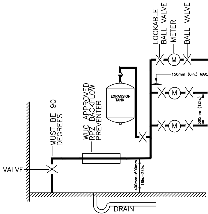
MULTIPLE METERS
