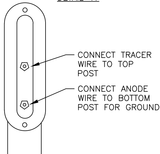
COBRA T2 TEST STATION
