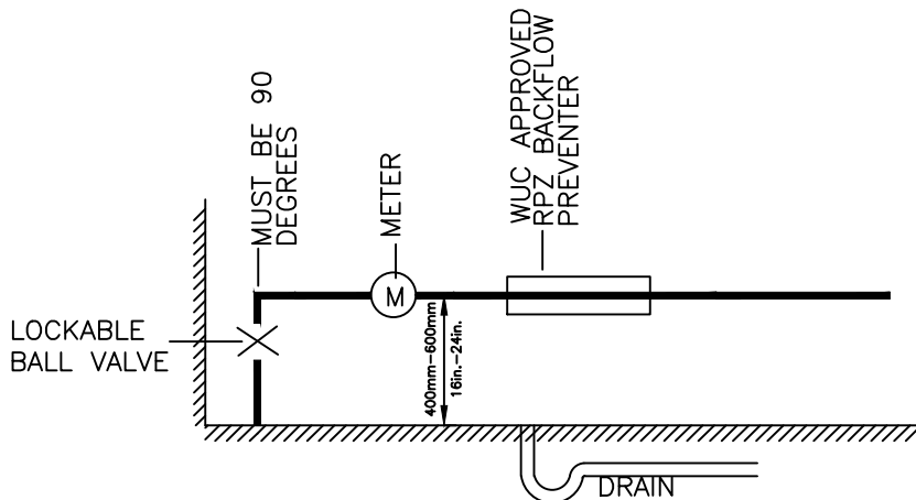
SINGLE METER
