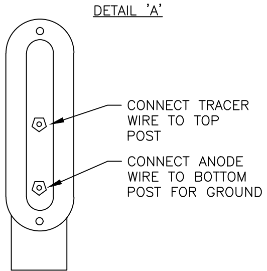
COBRA T2 TEST STATION
