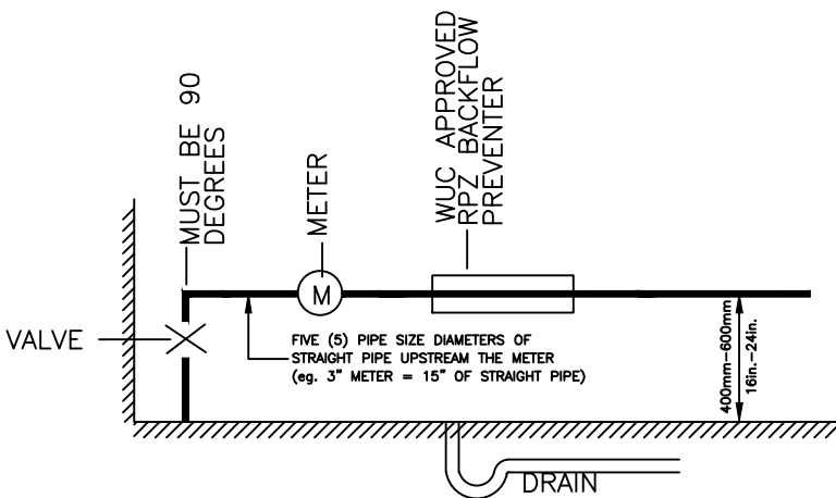
3" METER AND LARGER
