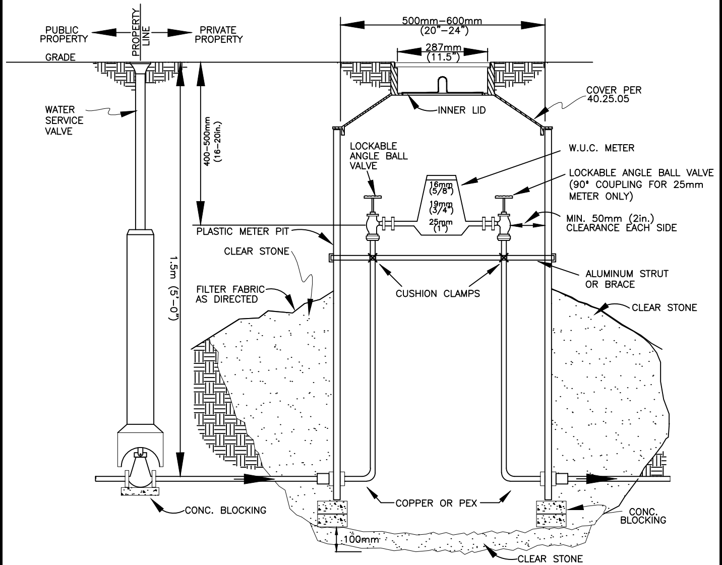
PRE-ASSEMBLED PIT
