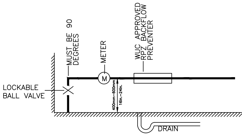
SINGLE METER (2" & SMALLER)
