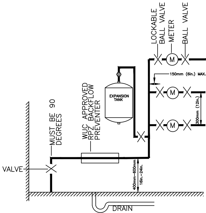
MULTIPLE METERS
