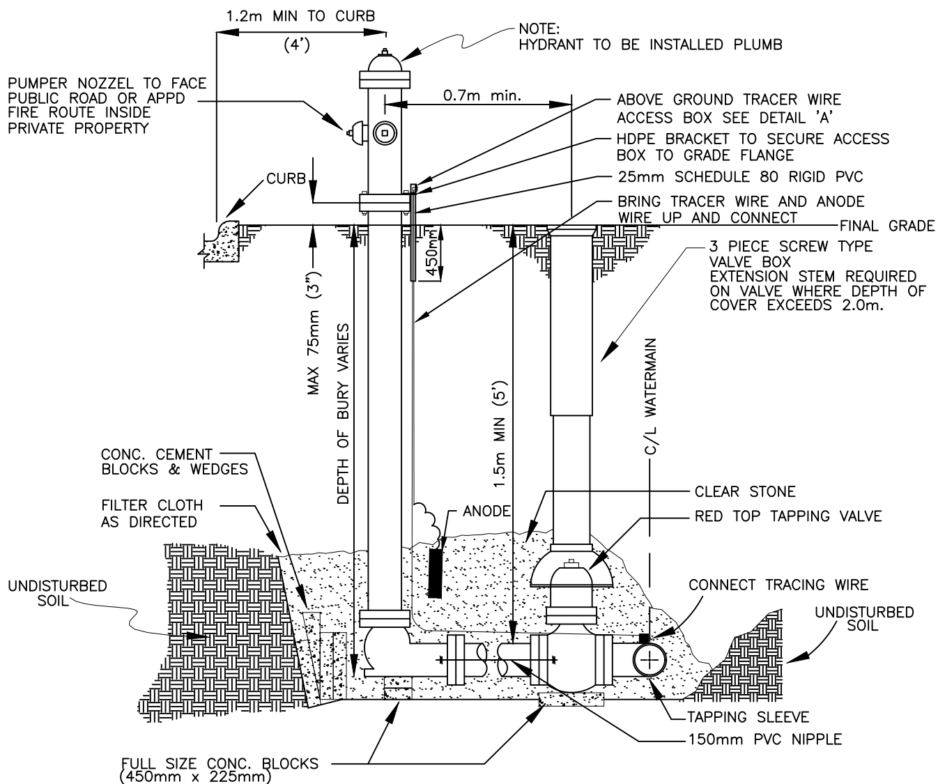
DETAIL 'A'
