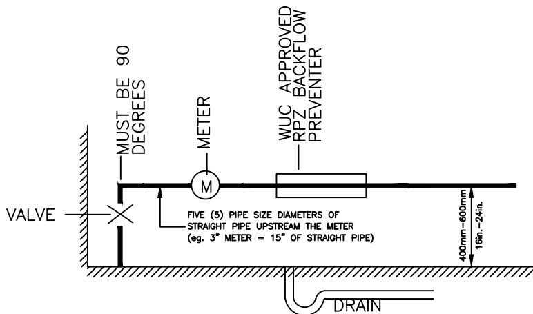
SINGLE METER (3" & LARGER)
