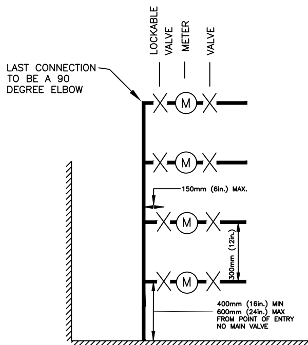
PROFILE VIEW
