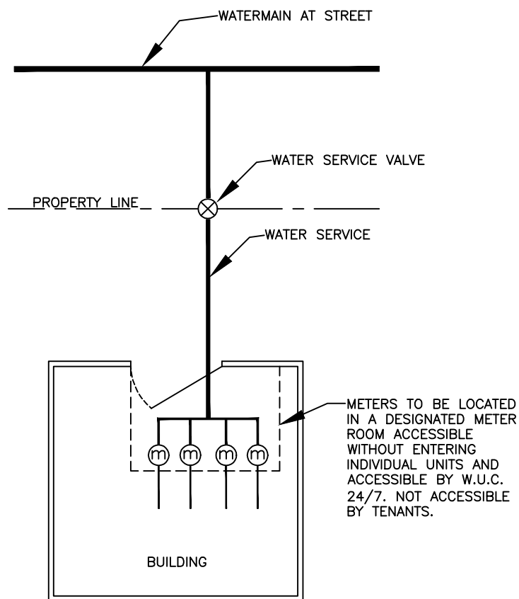
PLAN VIEW
